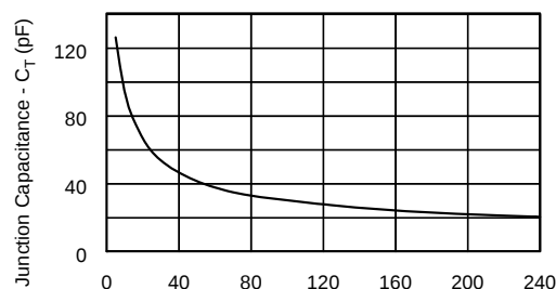
Typical Junction Capacitance
