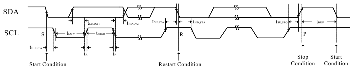
Figure 3 Interface Timing
