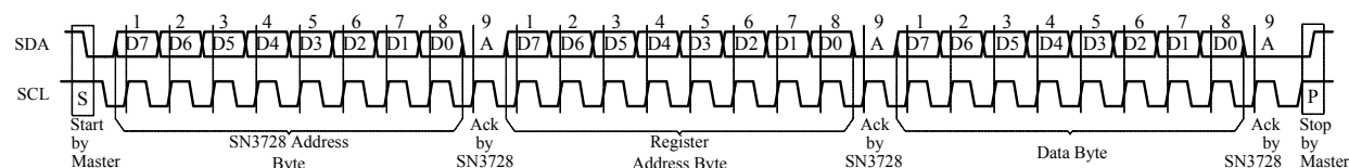
Figure 2 Writing to SN3728
