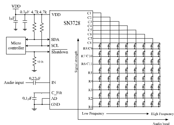
Figure 6 Audio EQ Mode
