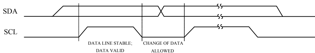
Figure 4 Bit Transfer
