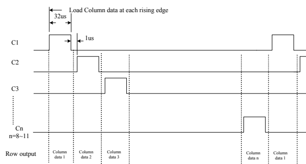
Figure 7 Dot Matrix Display Timing Diagram
