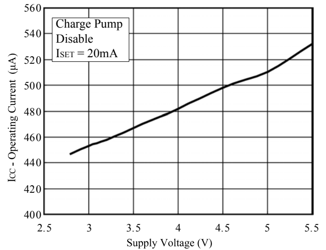
Figure 8 I_{CC} vs. Supply Voltage
