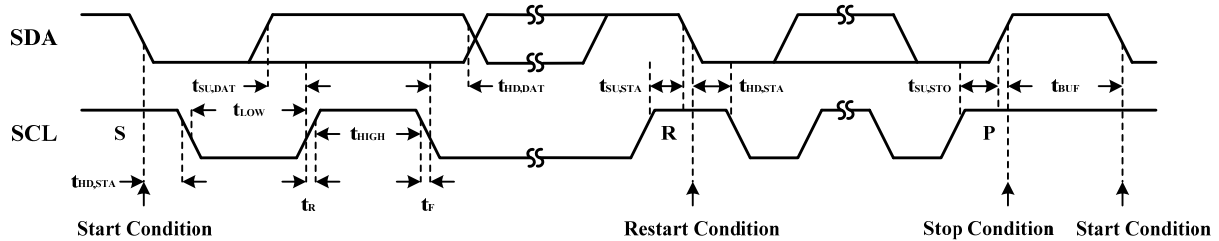
Figure 2 2-Wire Serial Interface Timing Details
