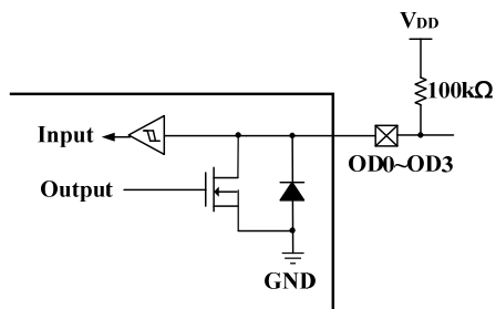
Figure 9 SN7328 Open-Drain I/O Ports Structure
