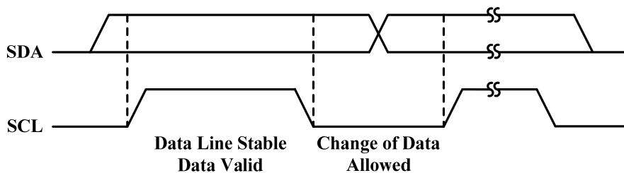
Figure 4 Bit Transfer
