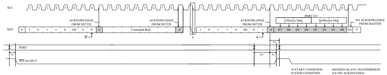
Figure 7 Reading I/O Ports of SN7328
