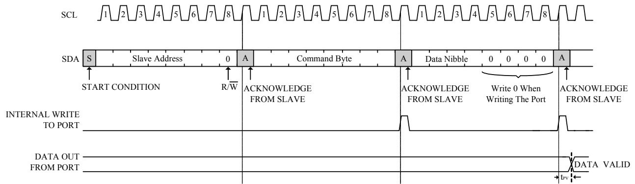
Figure 6 Writing to the SN7328
