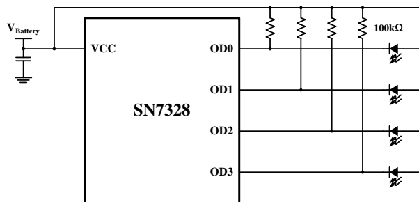
Figure 10 Driving LEDs with OD Ports
