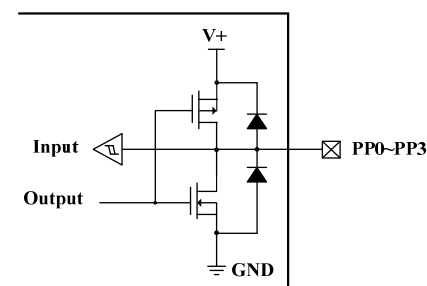
Figure 8 SN7328 Push-Pull I/O Ports Structure
