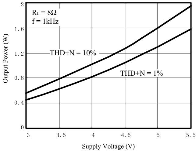
Figure 18 Output Power vs. Supply Voltage
