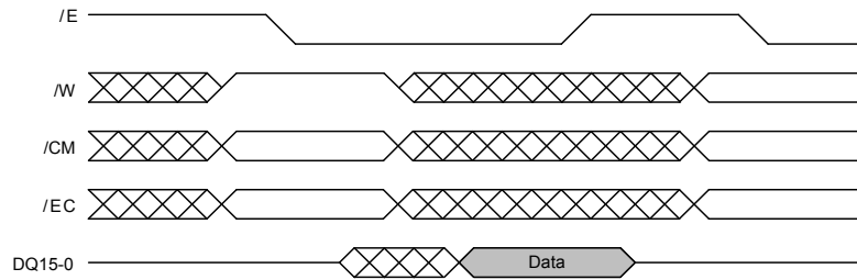
Figure 6: Read Cycle
