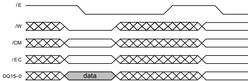
Figure 7: Write Cycle
