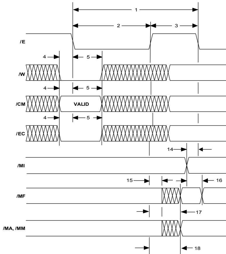
Figure 14: Compare Cycle
