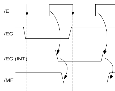
Figure 9: /EC (Int) Timing Diagram
