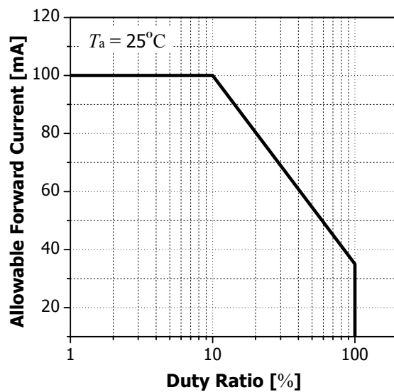
Allowable Forward Current vs. Duty Ratio
