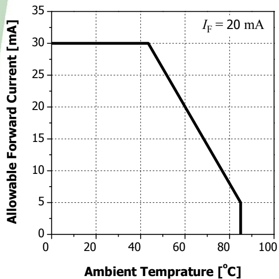
Allowable Forward Current vs. Ambient Temperature
