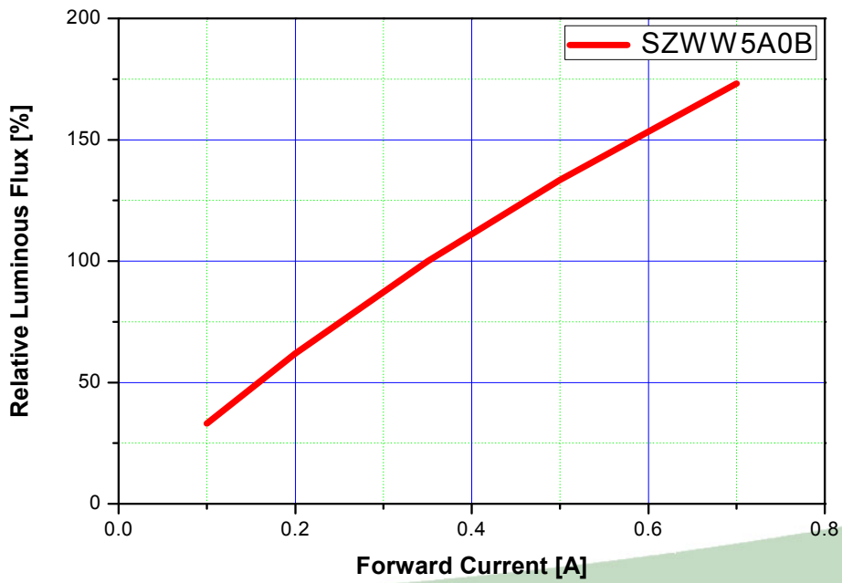
Forward Current vs. Normalized Relative Luminous Flux, Ta=25℃
