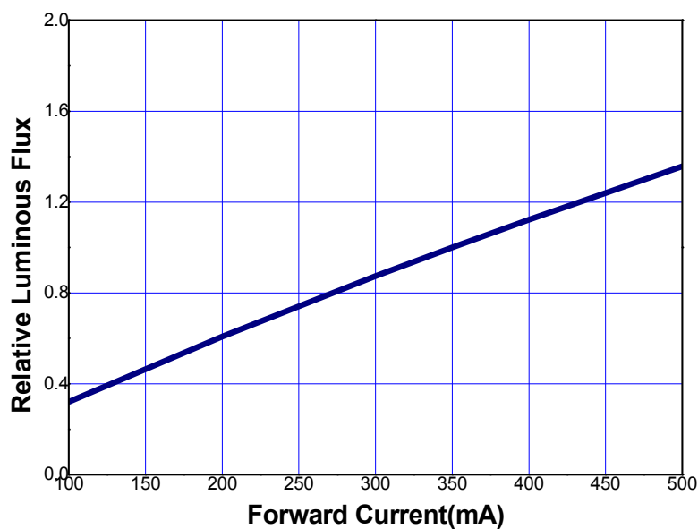
Normalized Relative Luminous Flux vs. Forward Current, T_a=25^\circ\text{C}
