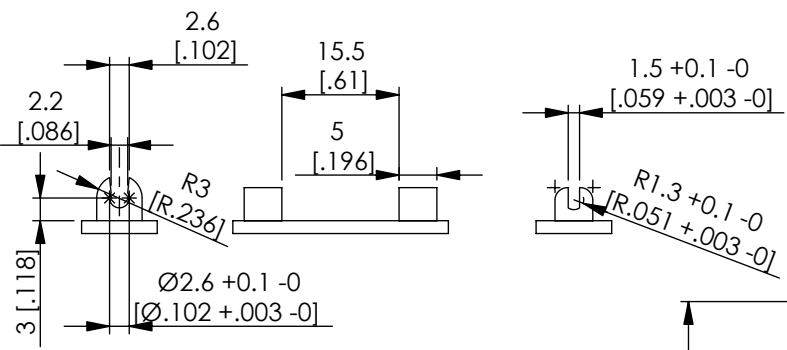
RECOMENDED SHAFT FIXTURE SHAPE
