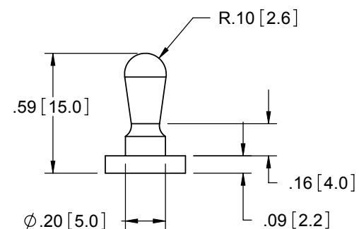
P/N: CS-113-2 STRIKER 1. MATERIAL: SUPERTOUGH NYLON 6/6 (RMS-73). 2. COLOR: BLACK.
