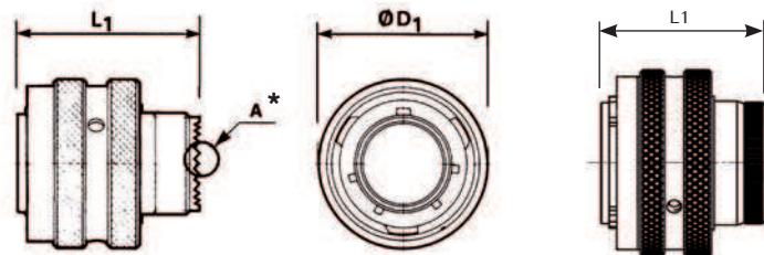
Type 5
