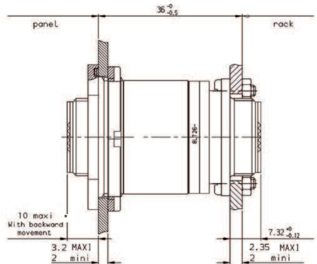
Mated connectors
