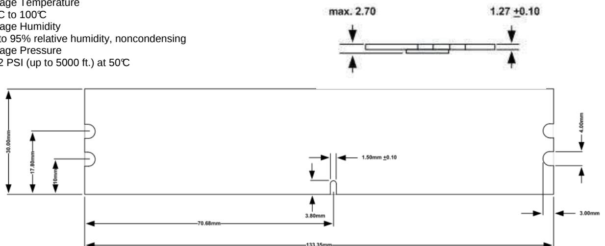
Figure: mechanical dimensions 1
