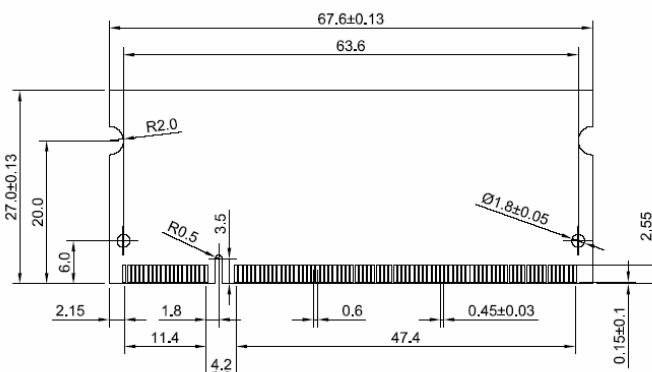
Figure 1: Mechanical Dimensions
