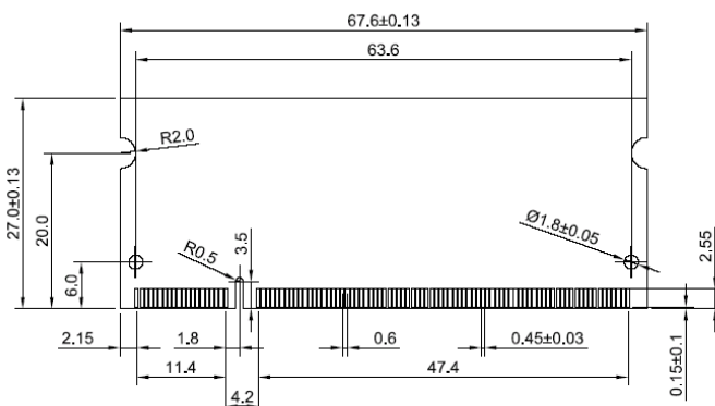
Figure: Mechanical Dimensions
