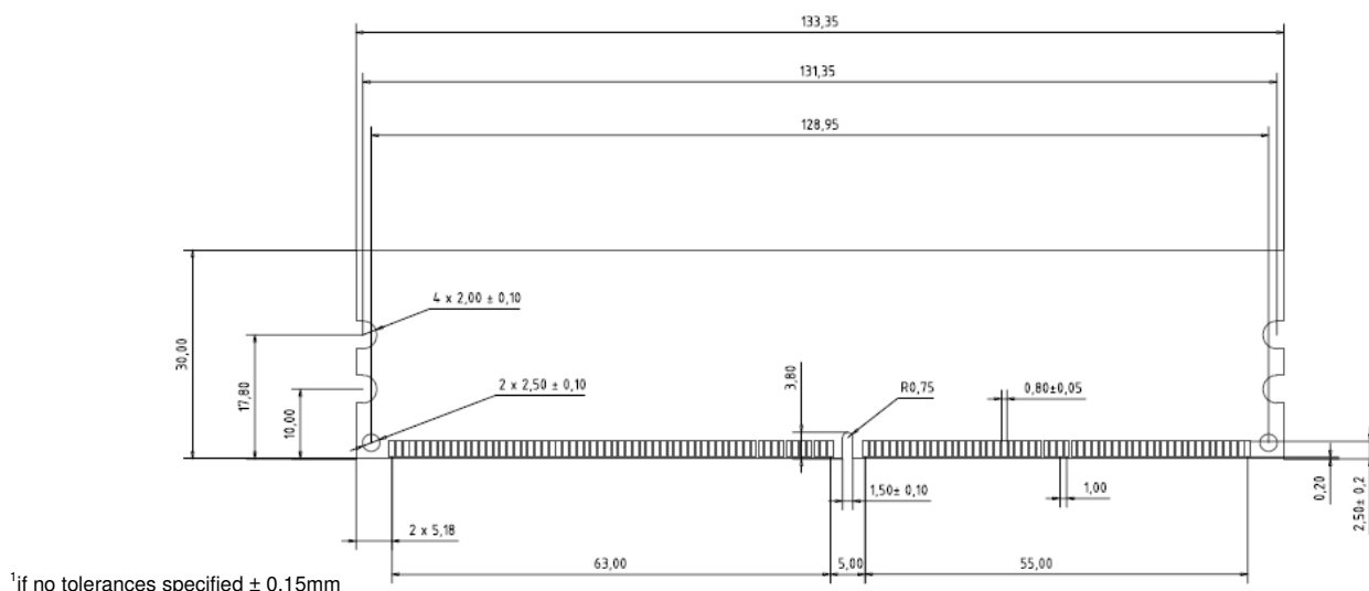
Figure: mechanical dimensions 1
