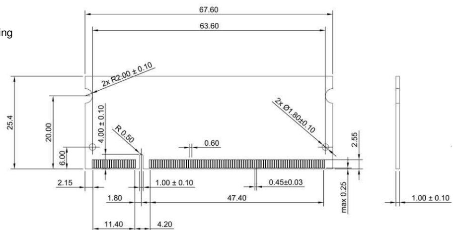
Figure: mechanical dimensions 1
