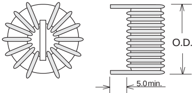
Style 'OH' - Horizontal Mount
