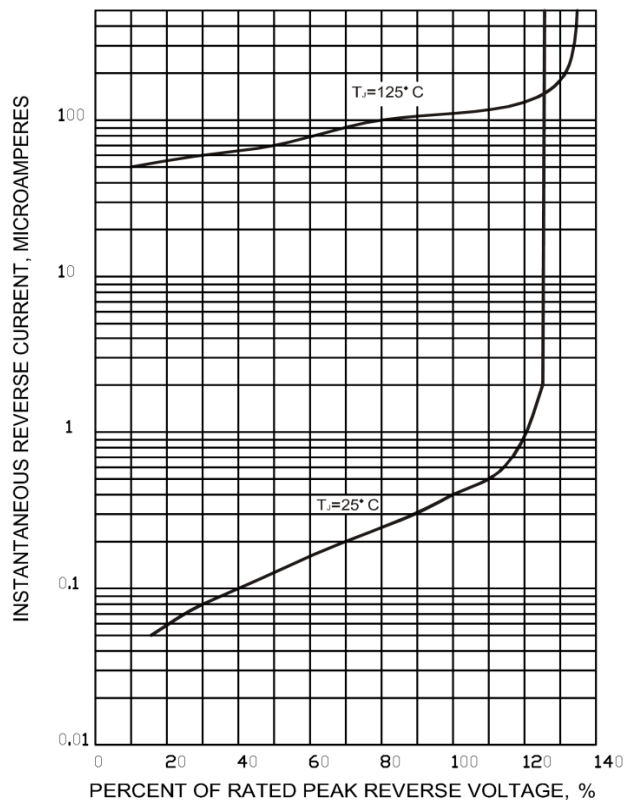
FIG.6-TYPICAL REVERSE LEAKAGE CHARACTERISTICS PER LEG
