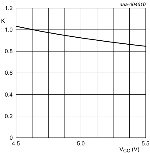
K-factor for 74HCT132-Q100
