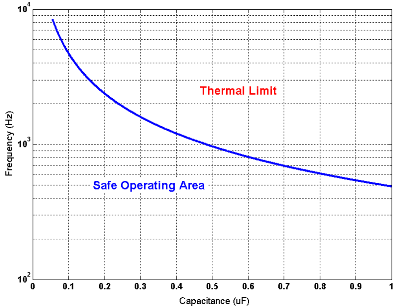
Figure 3: Thermal shutdown boundary as function of frequency and load capacitance for a full-scale ( \pm 200V ) output signal. Operation in the shutdown range is permitted only for short durations. Signal distortion or a blown fuse may occur.
