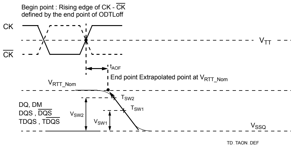
Figure 15. Definition of tAOF
