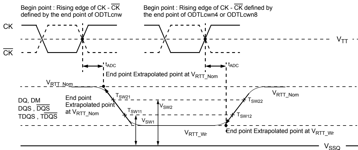
Figure 17. Definition of t_{ADC}
