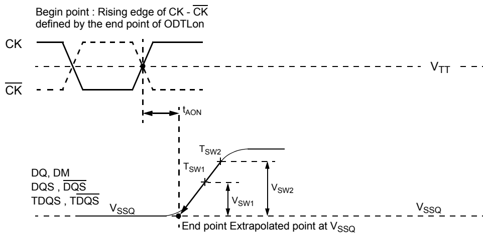
Figure 13. Definition of tAON
