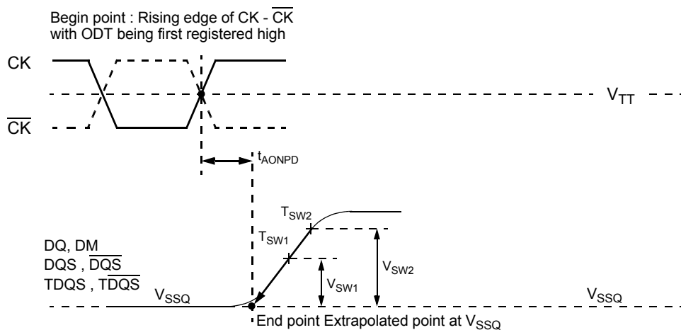
Figure 14. Definition of tAONPD
