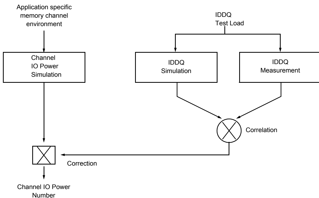
Figure 19. Correlation from simulated Channel IO Power to actual Channel IO Power supported by IDDQ Measurement.
