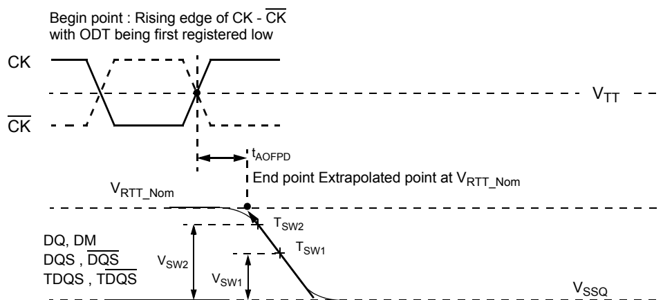
Figure 16. Definition of t_{AOFPD}
