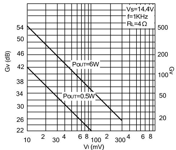
Fig. 21 Gain versus Input Sensitivity (Stereo amplifier)
