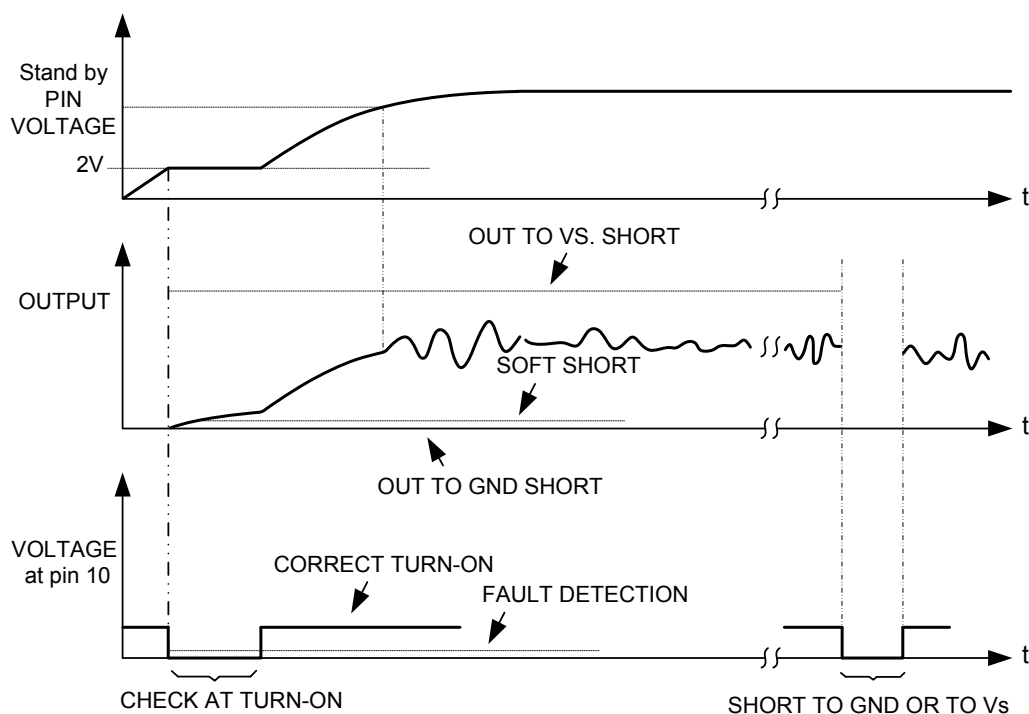
Fault Waveforms
