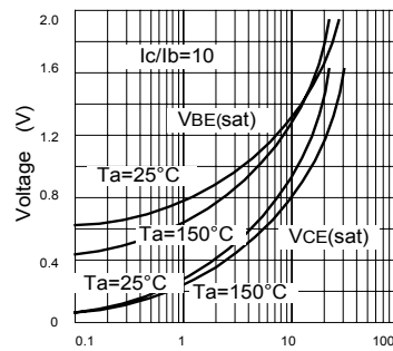
Figure 6 "ON" Voltage
