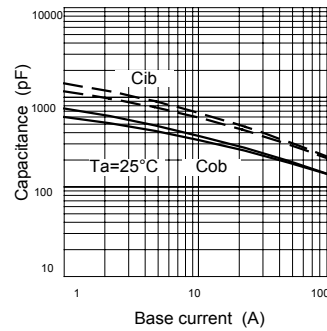
Figure 10 Capacitances
