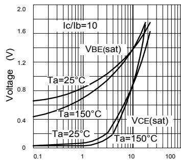
Figure 5 "ON" Voltage
