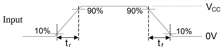
VOLTAGE WAVEFORMS INPUT RISE AND FALL TIMES
