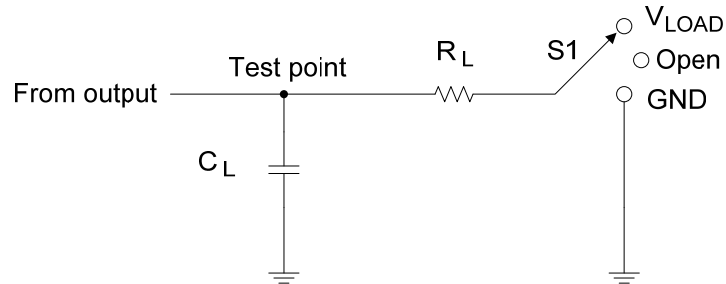
TEST CIRCUIT
