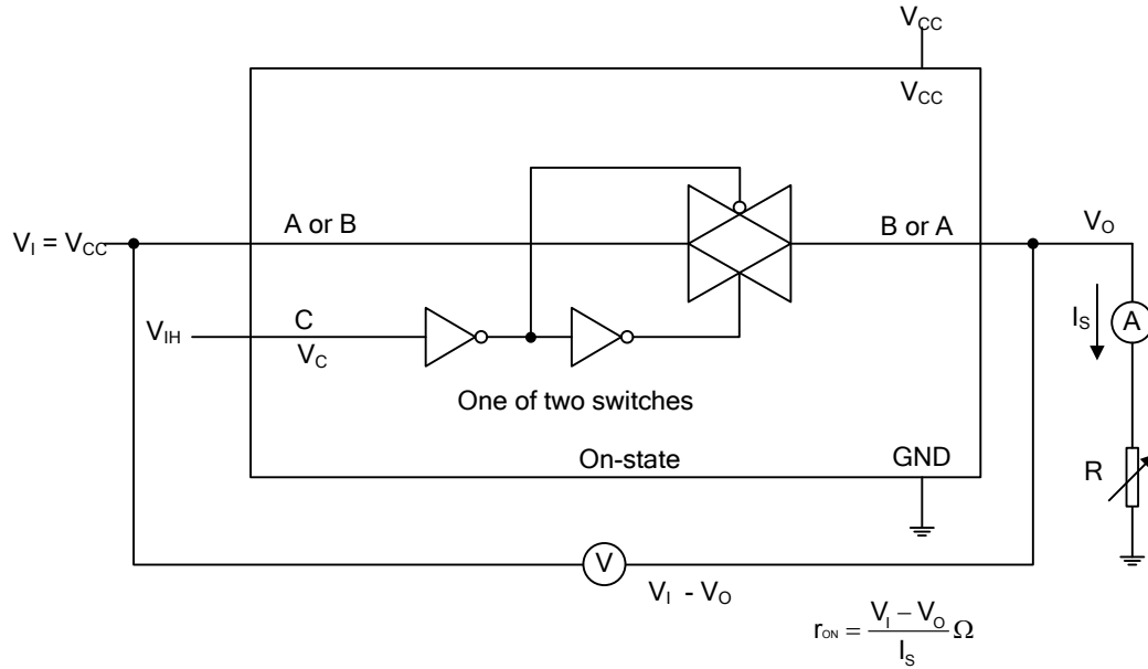
Fig.1 On-state resistance test circuit
