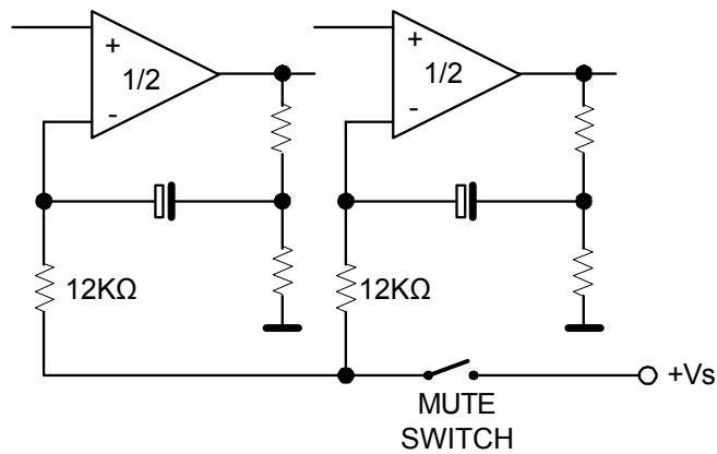
Figure 1. Example of Muting Circuit
