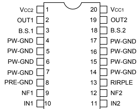
FOR SOP-20
