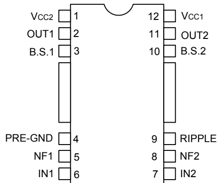
FOR DIP-12H
