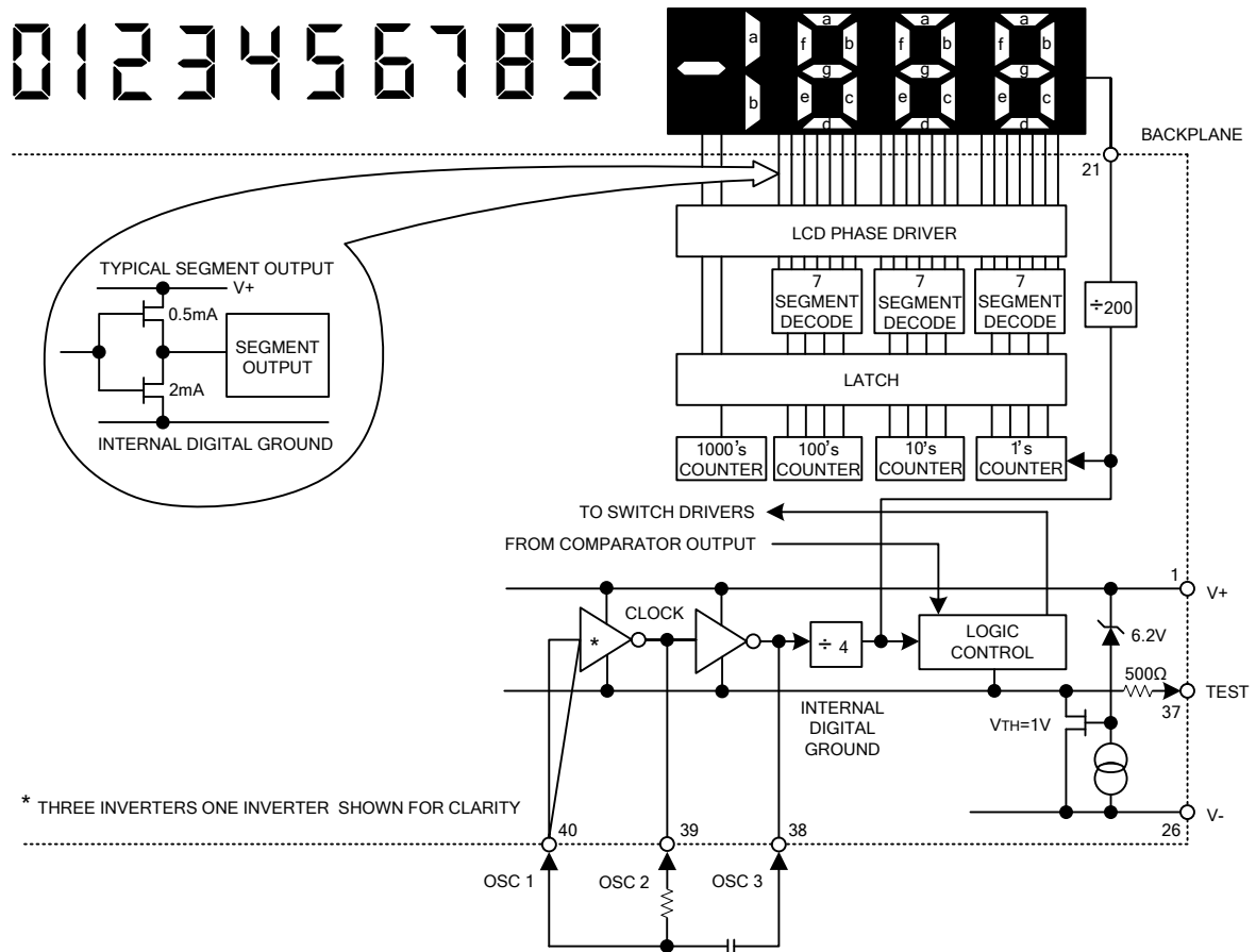
Fig.5 Digital Section
