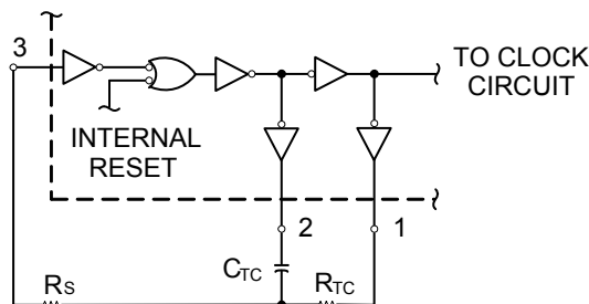
Oscillator Circuit Using RC Configuration
