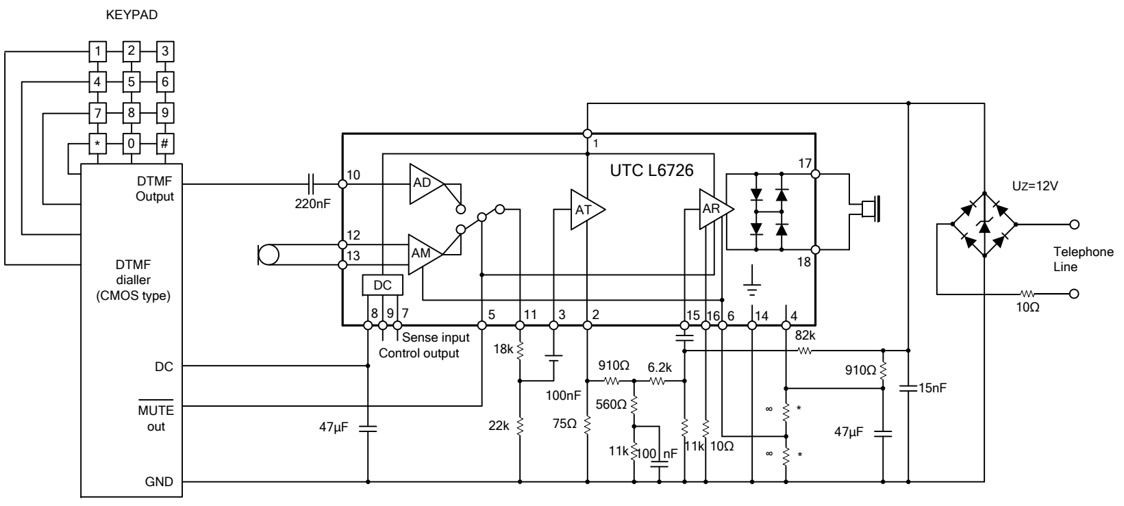
Fig. 6 Typical tong dialling telephone
