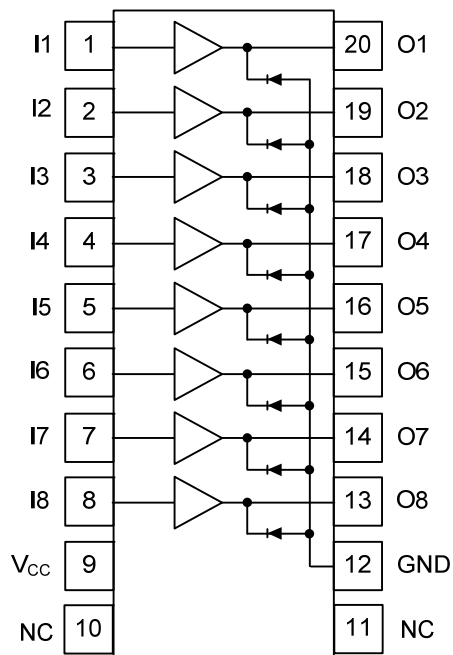
SOP-20
