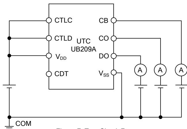
Figure 7. Test Circuit 7
