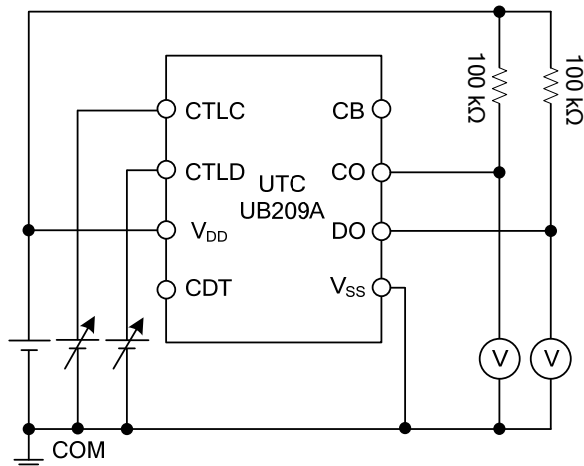
Figure 4. Test Circuit 4
