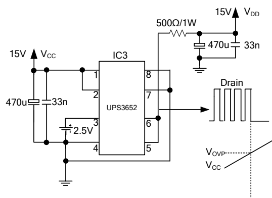
FIG.9 OVP test circuit
