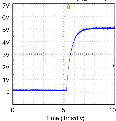
Feedback Voltage During Loadjump From 10% Up To 100% Load ( V_{AC}=264V )
