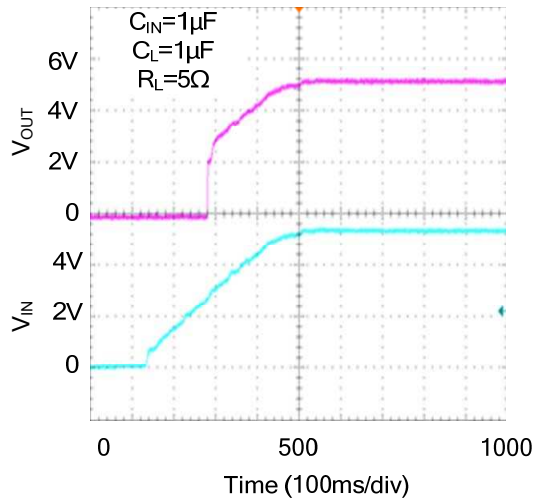
UVLO protection at rising
