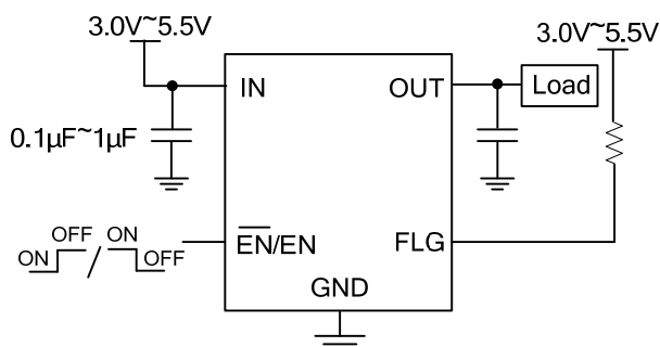
Figure 1. Supply Bypassing
