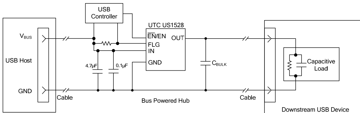
Figure 2. Soft Start
