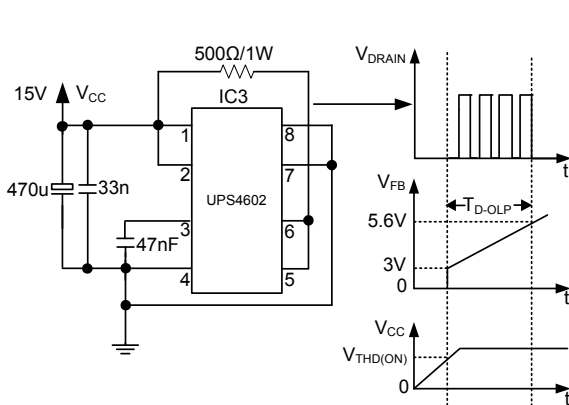
FIG.8 OLP test circuit
