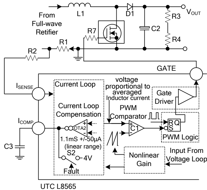
UTC L8565 Fig. 10 Complete System Current Loop
