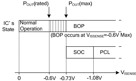
Fig. 8 BOP, SOC and PCL Protection as Function of V_{SENSE}
