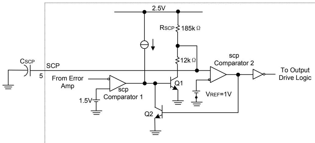
Fig. 3 SCP Circuit
