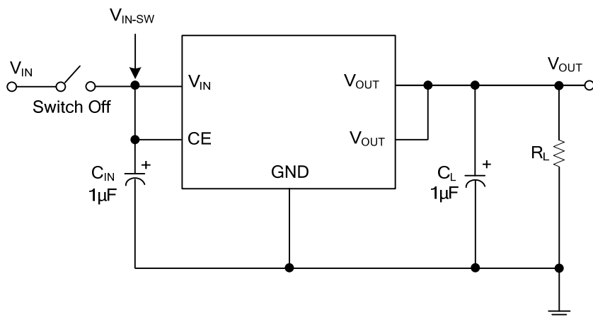
Test Circuit 1
