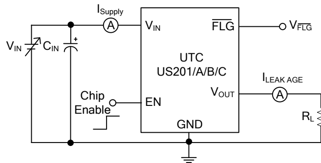
Fig.2 Supply Current
