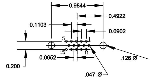
15 POSITION FEMALE
