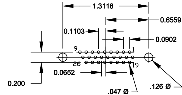
26 POSITION FEMALE
