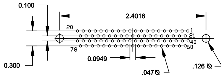
78 POSITION FEMALE
