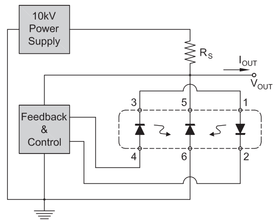
Typical HV Linear Regulator Circuit
