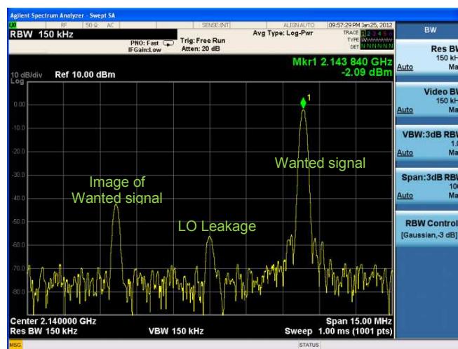
Figure 8 Transmitter Output, when NCO BIN is Selected
