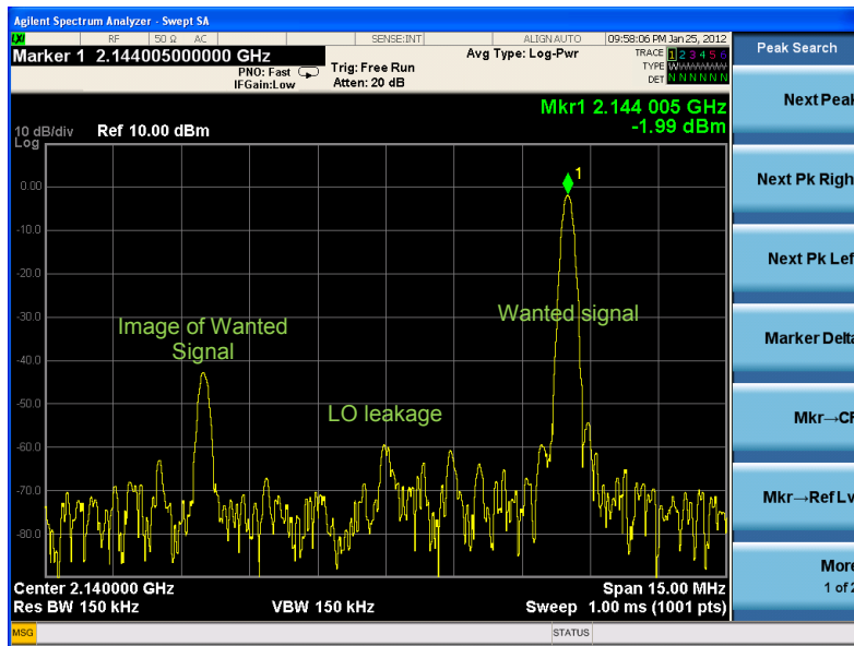
Figure 9 Transmitter Output, when NCO ALT 4MHz is Selected
