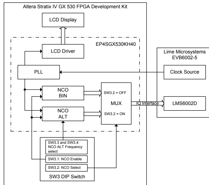
Figure 4 Test Project Block Diagram
