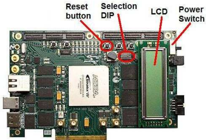
Figure 6 Key Components on Altera Stratix IV GX 530 FPGA Development Kit
