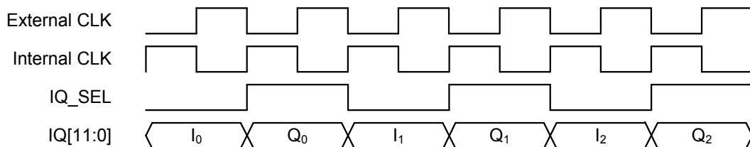
Figure 5 IQ Interface Data Align to the External Clock
