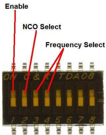
Figure 7 Selection DIP Used for NCO Control
