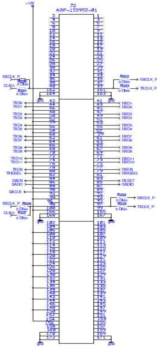
Figure 3 Connector J2 circuit diagram.
