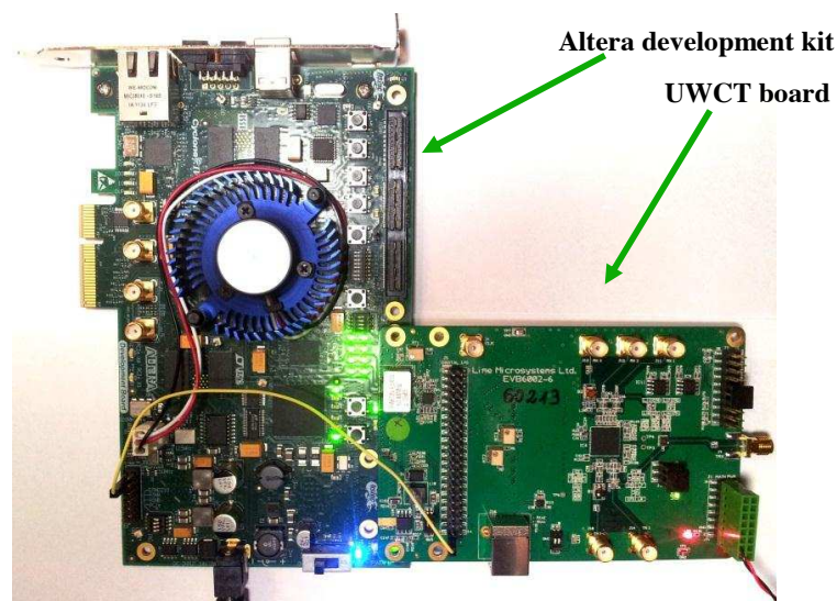
Figure 1 Altera development kit and UWCT board connection.
