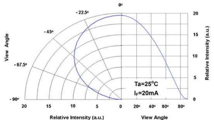
Radiation Pattern
