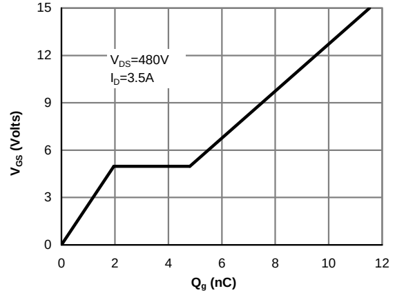
Figure 8: Gate-Charge Characteristics
