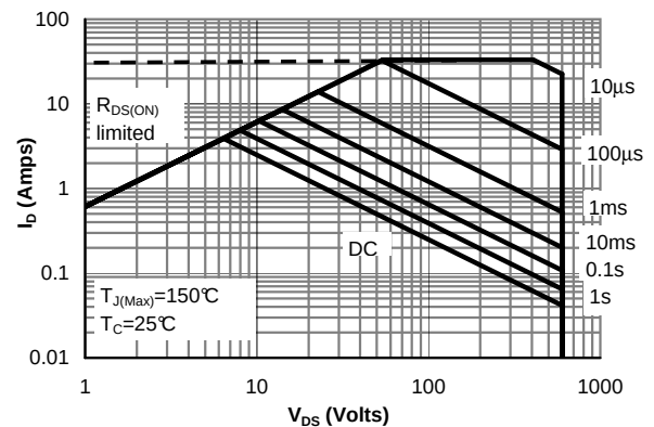
Figure 12: Maximum Forward Biased Safe Operating Area for AOTF7S60L (Note F)
