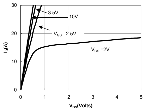
Figure 1: On-Regions Characteristic
