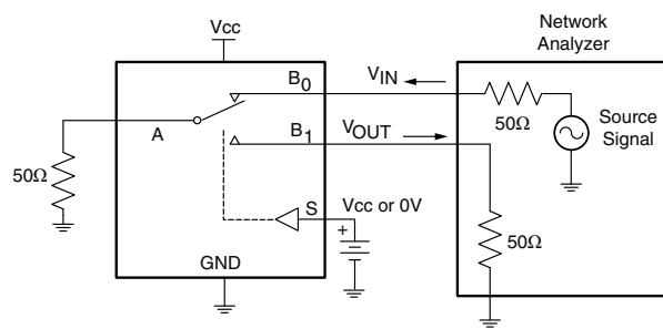
Figure 4. Crosstalk
