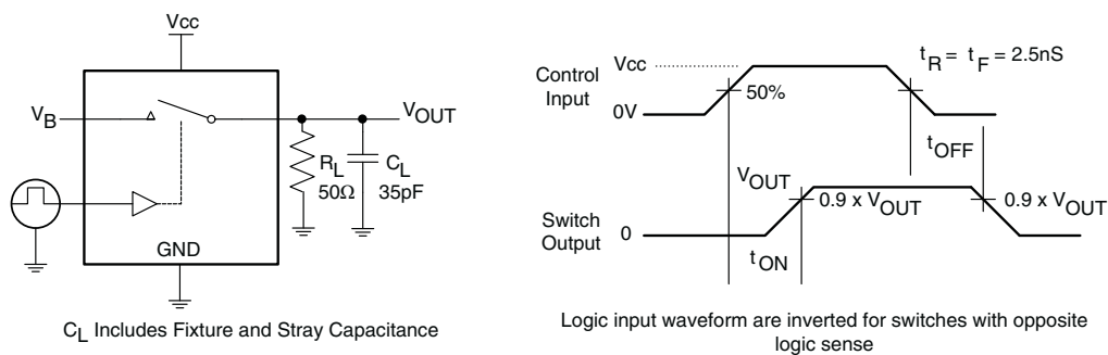
Figure 1. Turn-On/Turn-Off Timing
